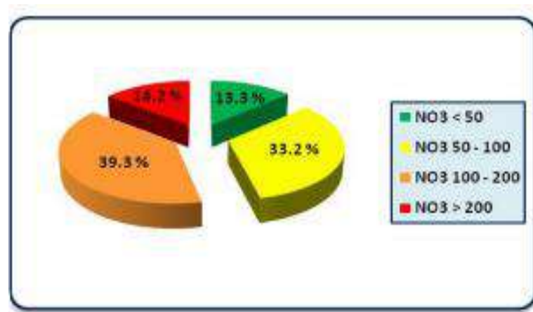
Figure 3.4: Nitrate Concentration in the Gaza Strip(PWA, 2014)
