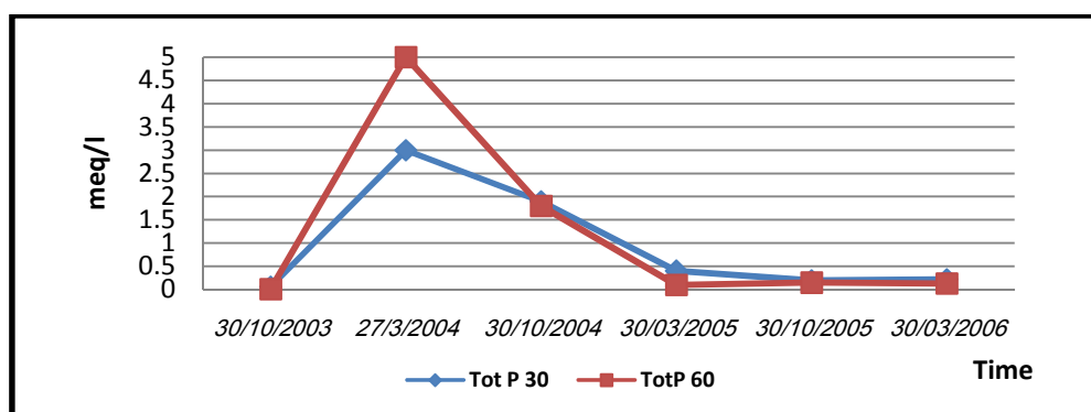
Figure 5-19: Phosphorus values for two soil layers.
