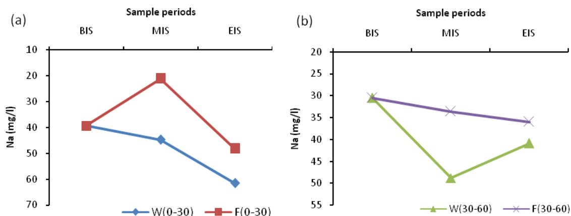
Figure 5.9: (a) 0-30cm, (b) 30-60 cm. \text{Na}^+ of soil layers for different irrigation water RWW and FW, (F= FW) and (W = RWW).
