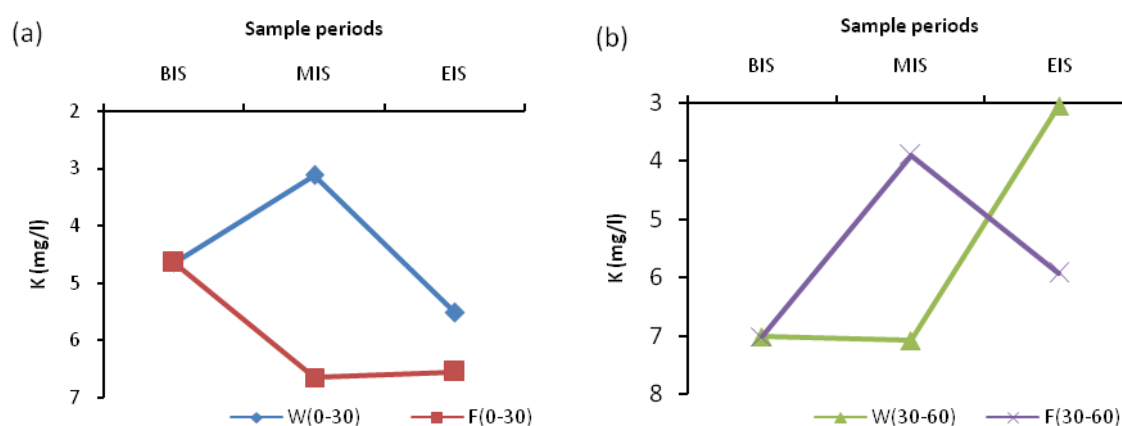
Figure 5.8: (a) 0-30cm, (b) 30-60 cm. \text{K}^+ of soil layers for different irrigation water RWW and FW, (F= FW) and (W = RWW).
