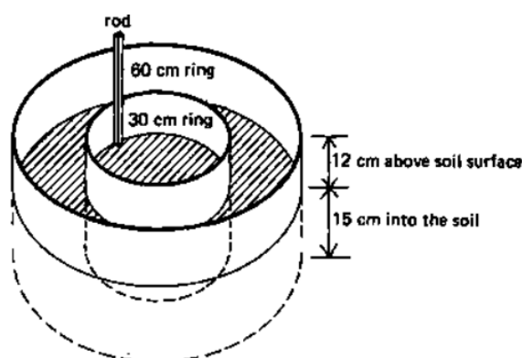
Figure 4.3: Double-ring infiltrometers (FAO, 1988)
