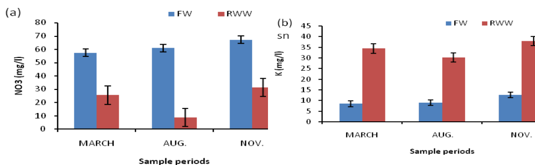
Figure.5.4: NO 3 - (a) and K + (b), concentration during sampling periods
