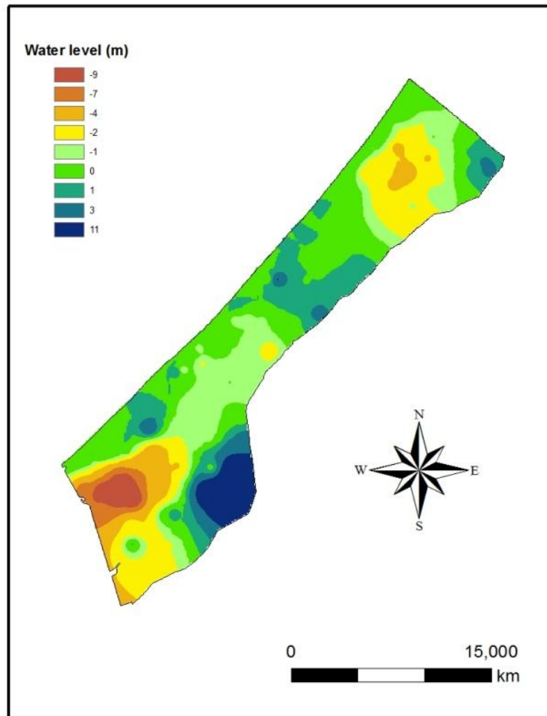
Figure 3.4: Contour map of groundwater level for year 2008 (prepared by Researcher).
