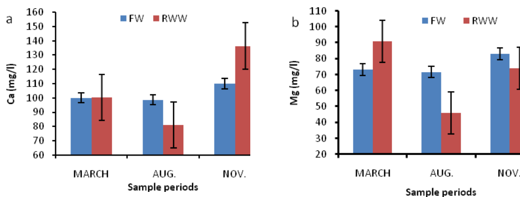
Figure.5.3: Ca^{+2} (a) and Mg^{+2} (b), concentration during sampling periods
