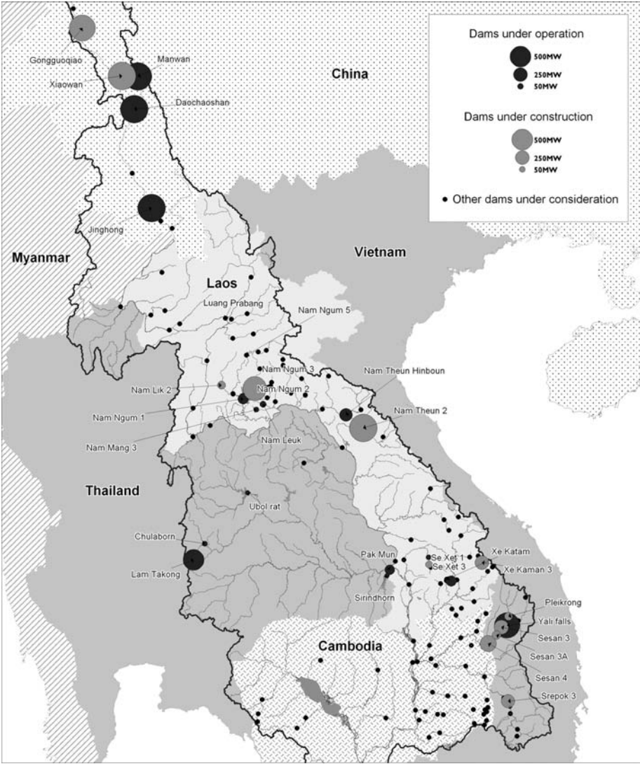
Figure 2.2 Location of dams in operation and under construction in the Mekong Basin
