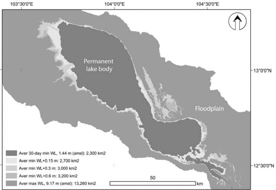
Figure 9.1 Inundated areas due to the increased dry season water level
