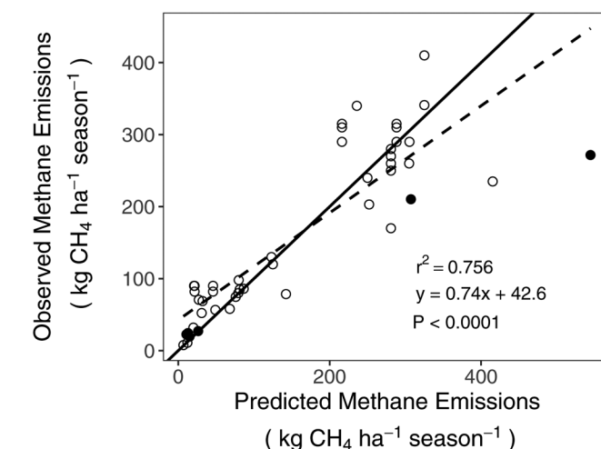
Fig. 6. The relationship between the observed versus predicted \text{CH}_4 emissions when using one (open circle) or two (closed circle) practices to adjust average emissions. The solid line is the 1:1 line, and the dashed line is the best fit line through all points.
