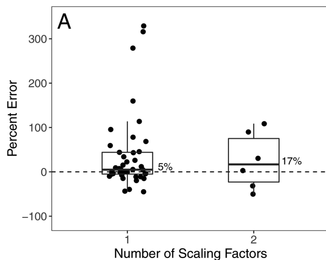
Fig. 7. (A) The percentage error [(\text{observed } \text{CH}_4 - \text{predicted } \text{CH}_4) / \text{predicted } \text{CH}_4] for one and two scaling factors. Data points are staggered for visual interpretation. Points above the dashed line indicate that the observed \text{CH}_4 emissions were greater than the predicted \text{CH}_4 emissions and vice versa. A boxplot overlaying the data points indicates the median value (thick horizontal line), and the lower and upper lines of each box correspond to the first and third quartiles (the 25th and 75th percentiles). The whiskers extend from the hinge to the furthest value, but no further than 1.5 times the interquartile range (or the distance between the first and third quartiles) from the hinge. Data beyond the end of the whiskers are considered "outlying" points. (B) The percentage error [(\text{observed } \text{CH}_4 - \text{predicted } \text{CH}_4) / \text{predicted } \text{CH}_4] versus predicted \text{CH}_4 emissions.
