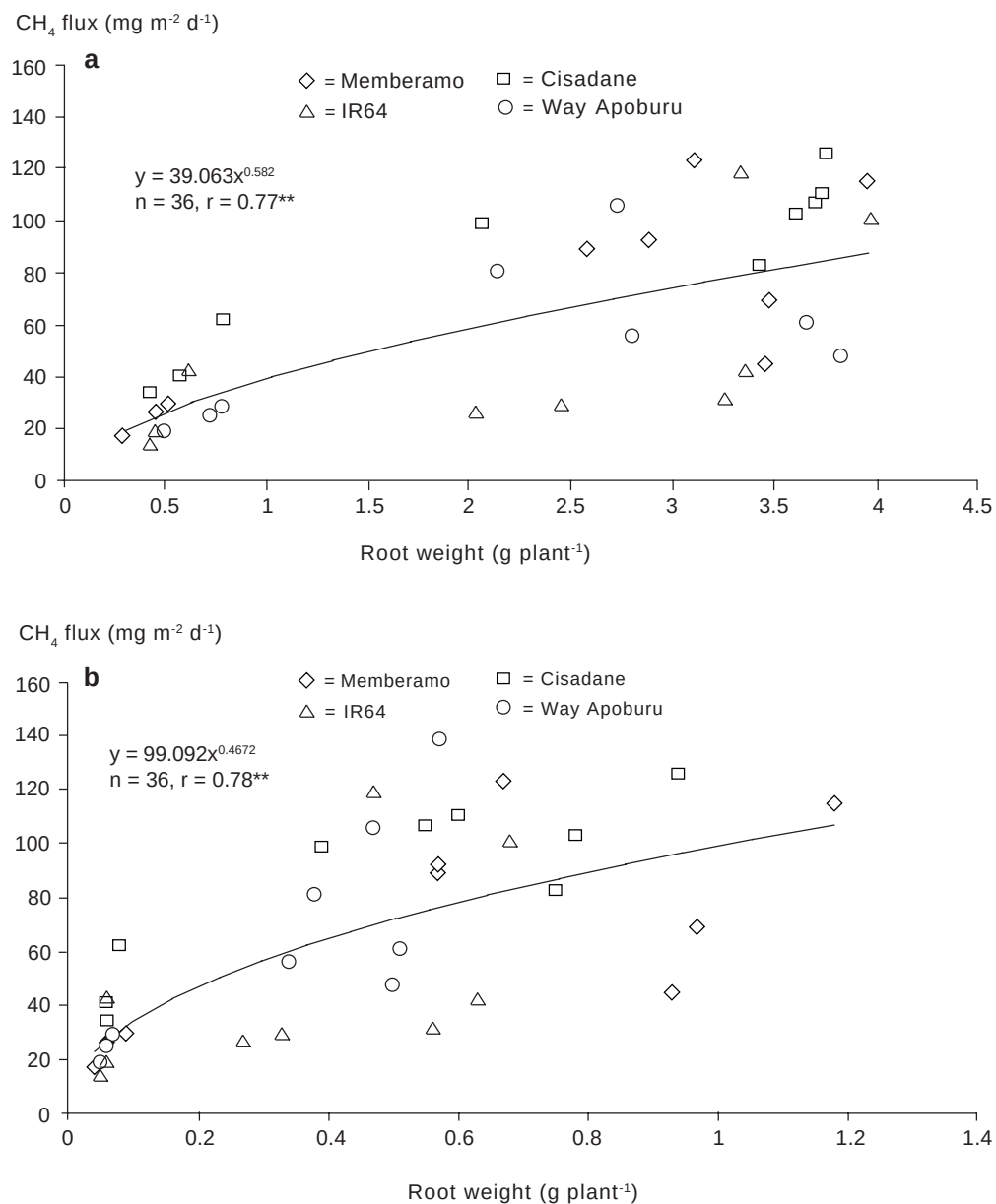
Fig. 5. Relationship between \text{CH}_4 flux and root dry weight of four rice cultivars, Jakenan Experimental Farm, Central Java, WS 2001/2004; root samples were taken from 0-10 cm (a) and 10-20 cm (b) (** indicate significant correlation at P < 0.01 ).
