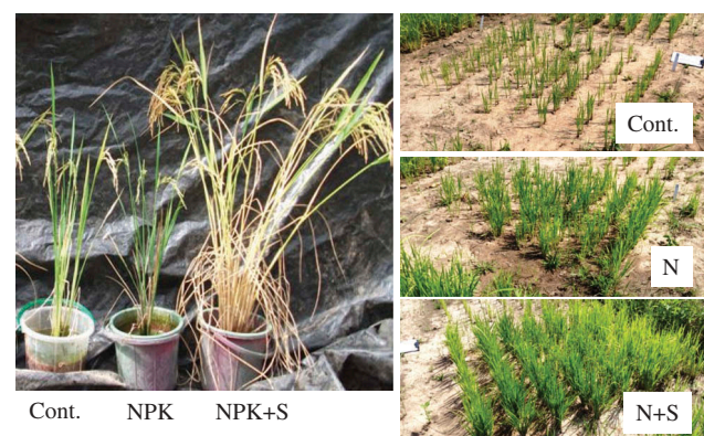
Figure 3. Significant responses to S application in S-deficient soils in the rainfed lowland of northern Ghana.
